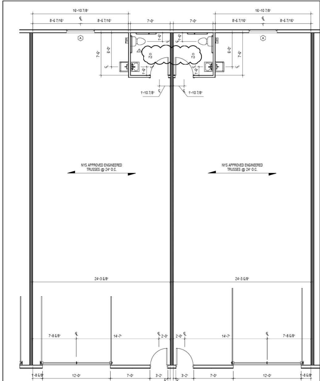
1 TYPICAL UNIT PLAN A4 1/4" = 1'-0"
